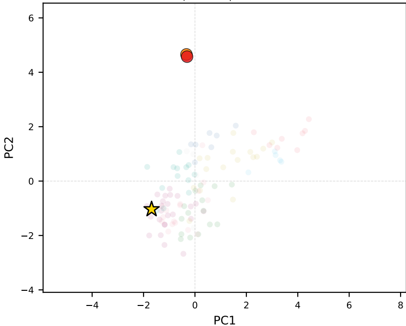
qwen3-1.7b | Palestine
