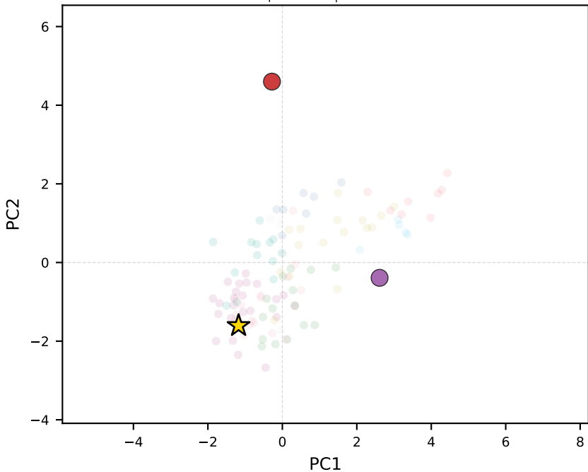
qwen3-1.7b | Rwanda
