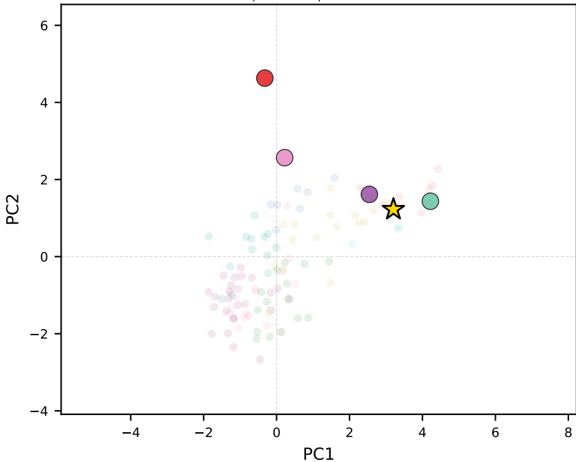
qwen3-1.7b | Switzerland
