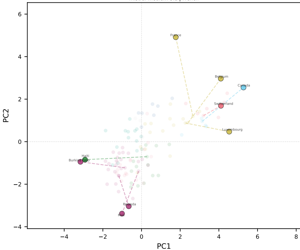
mistral-medium-3.1 | French
