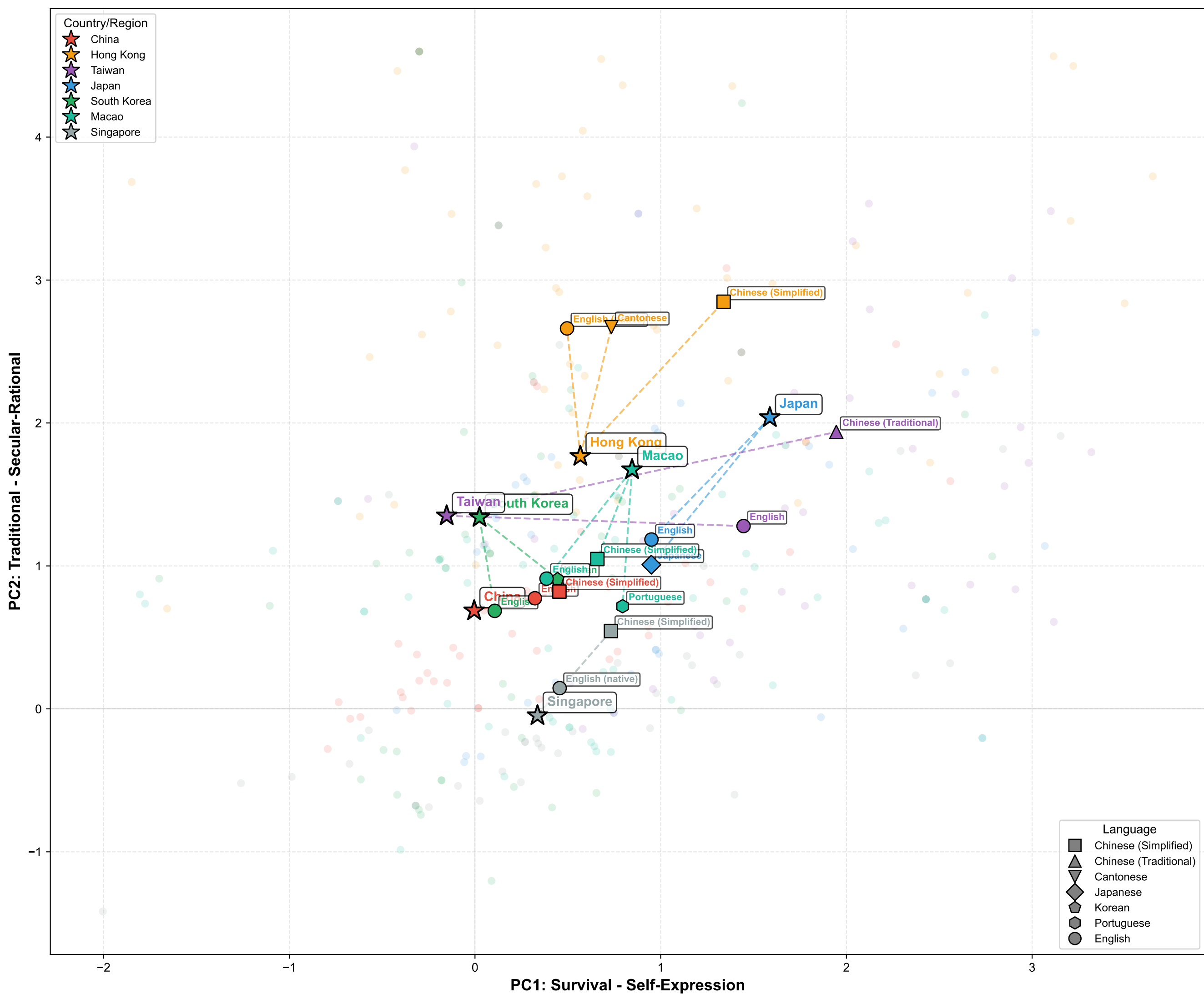
FigS6A: East Asia Cultural Coordinate Trajectory
