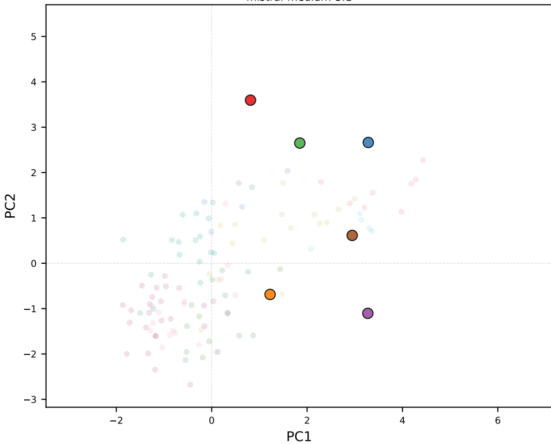
mistral-medium-3.1
