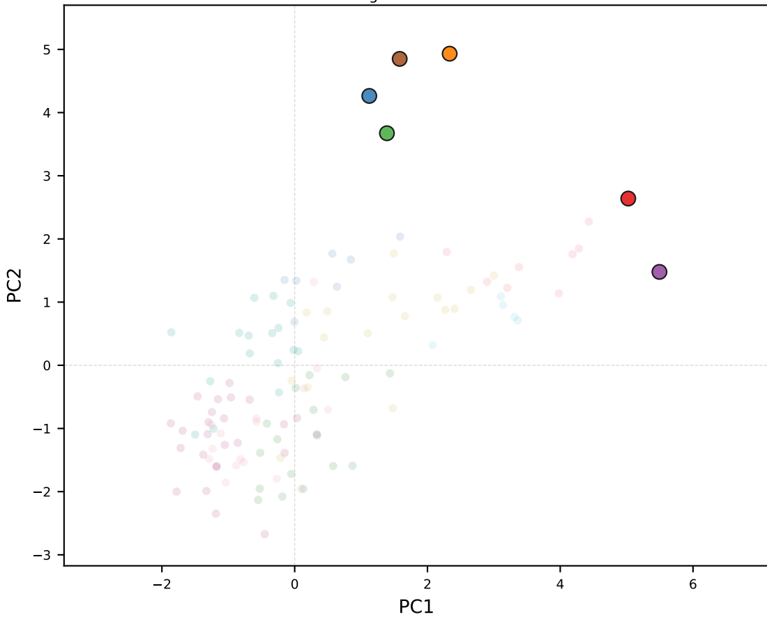
grok-4.1-fast
