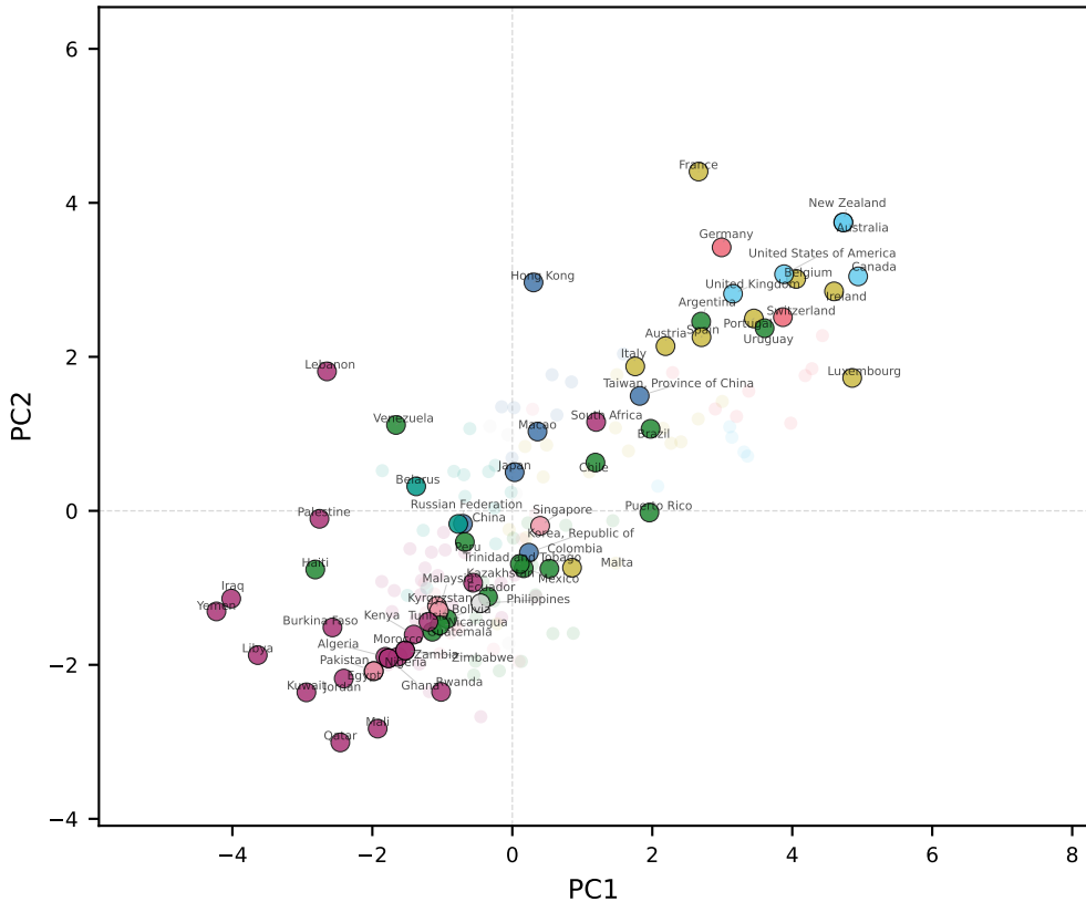
mistral-medium-3.1
