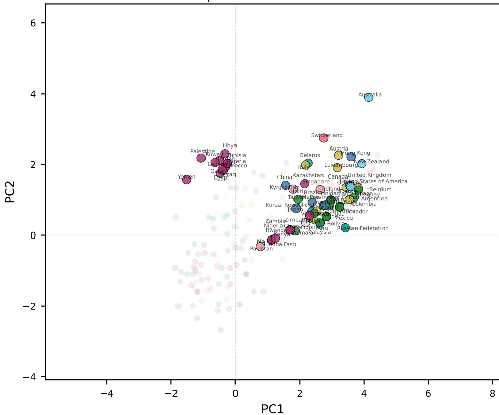
phi-3-mini-128k-instruct
