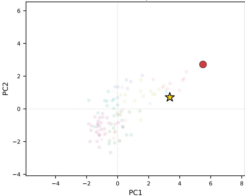
claude-sonnet-4.5 | Australia
