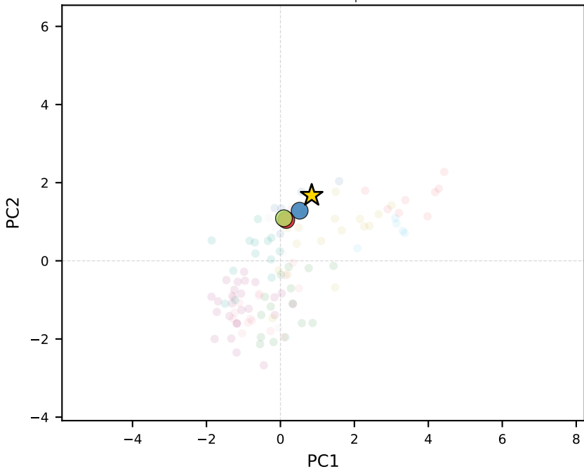
claude-sonnet-4.5 | Macao
