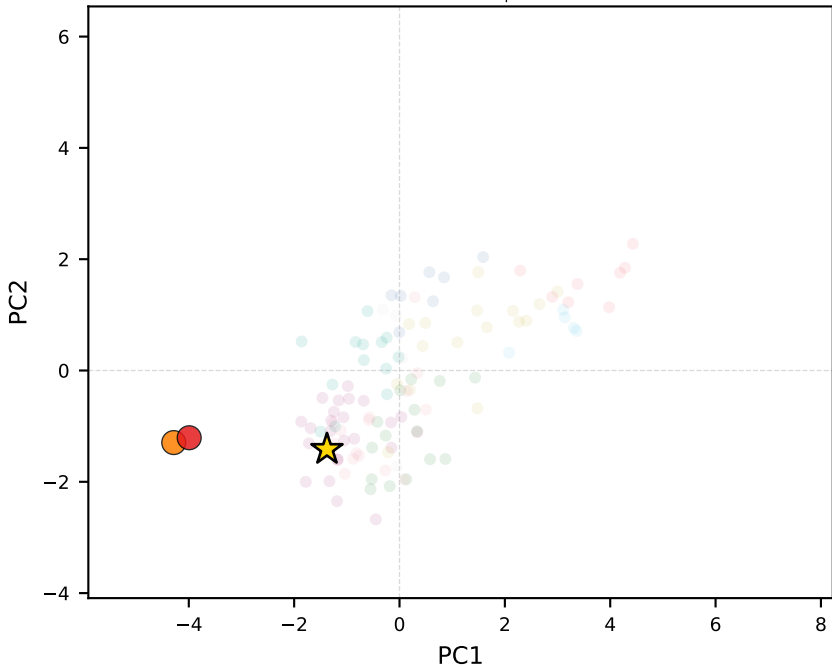
claude-sonnet-4.5 | Yemen
