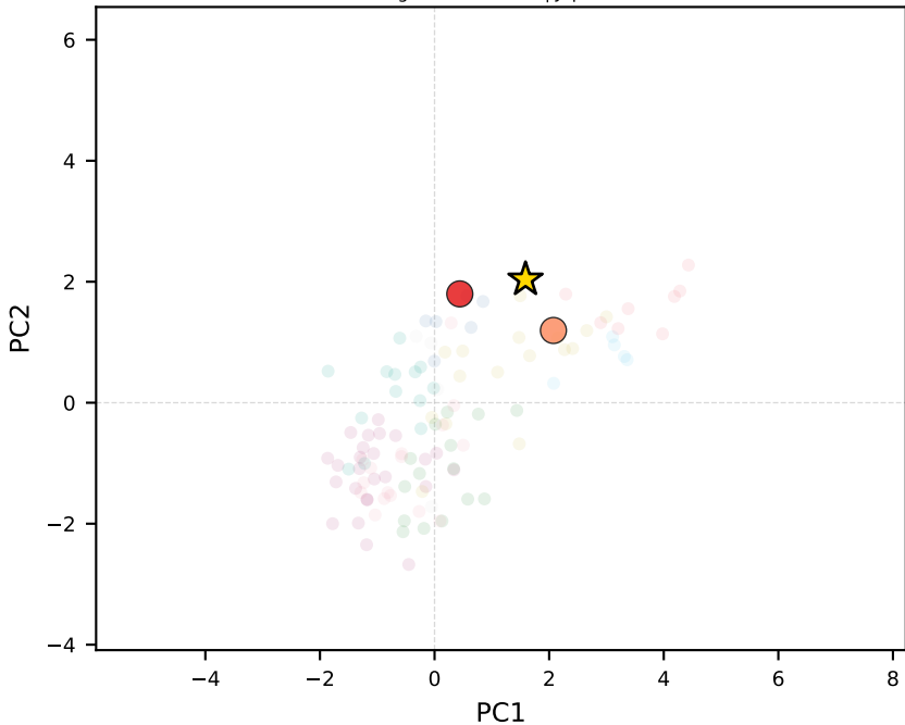
gemini-2.5-flash | Japan
