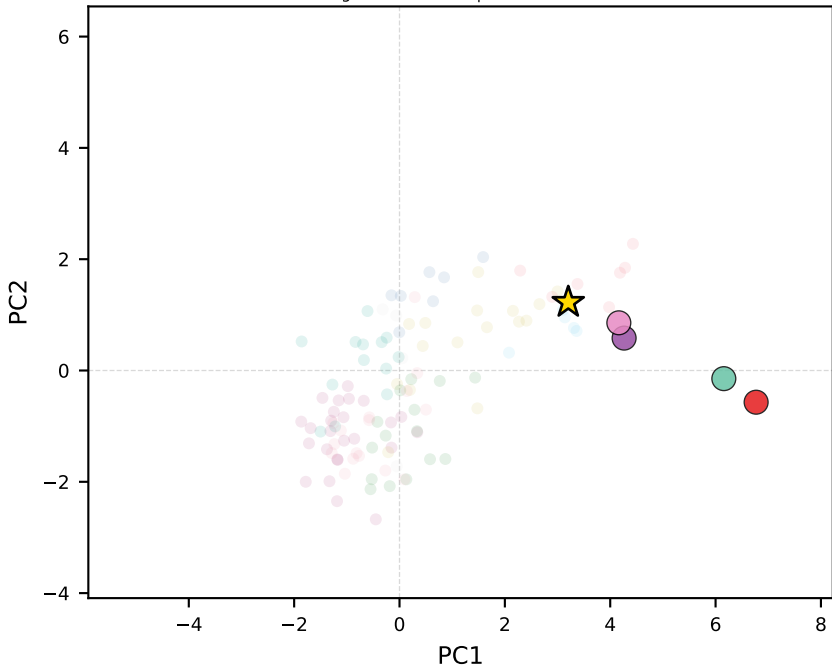
gemini-2.5-flash | Switzerland
