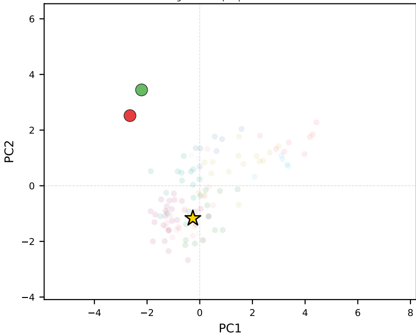
gemini-2.5-pro | Venezuela
