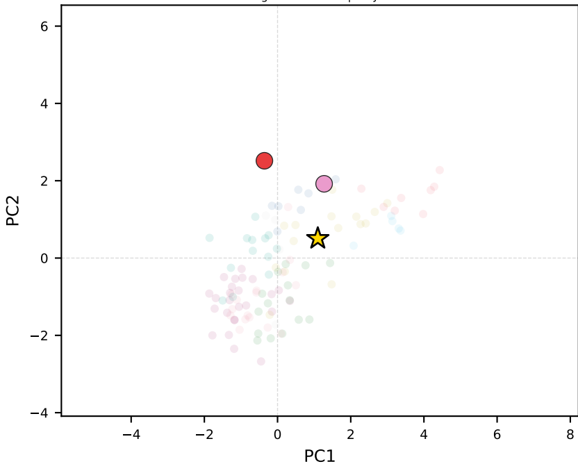
gemma-3-4b-it | Italy
