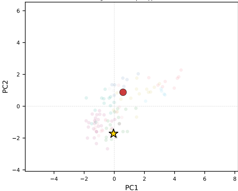
gemma-3-4b-it | Philippines
