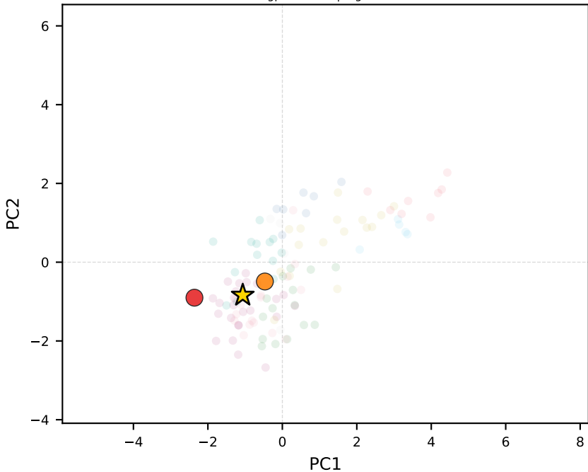
gpt-4o-mini | Algeria
