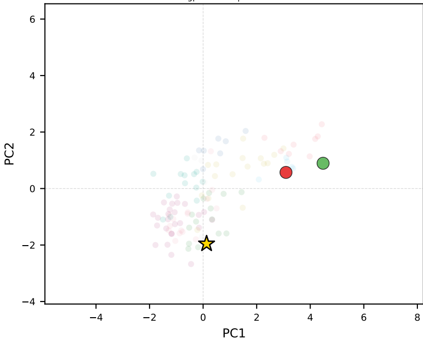
gpt-4o-mini | Colombia
