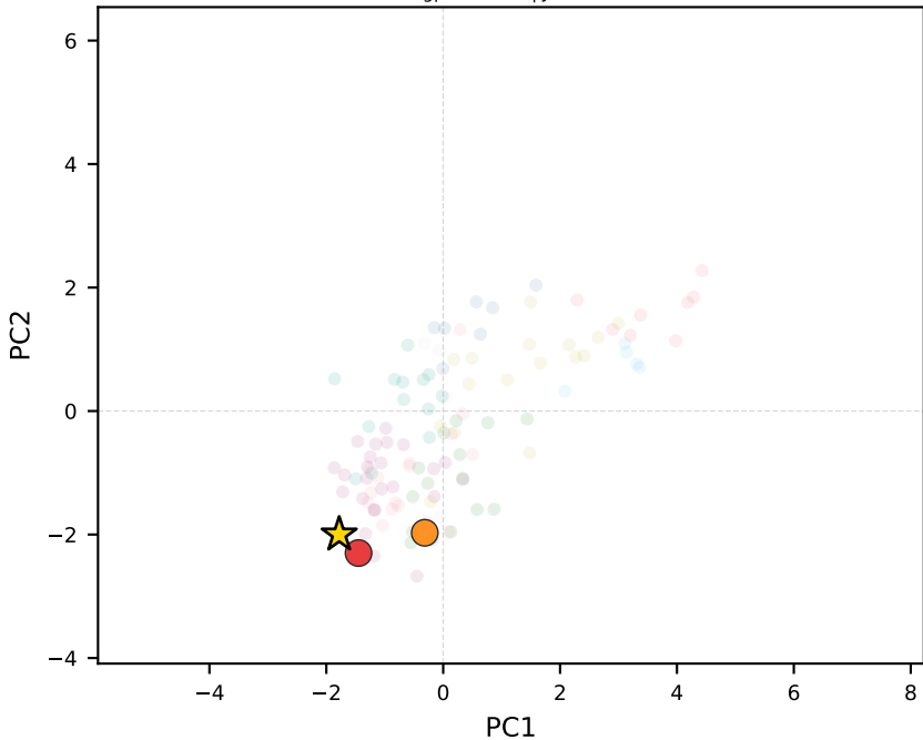
gpt-4o-mini | Jordan
