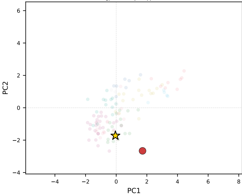
gpt-4o-mini | Philippines
