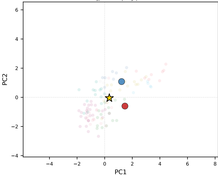
gpt-4o-mini | Singapore
