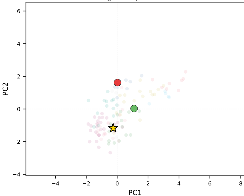
gpt-4o-mini | Venezuela
