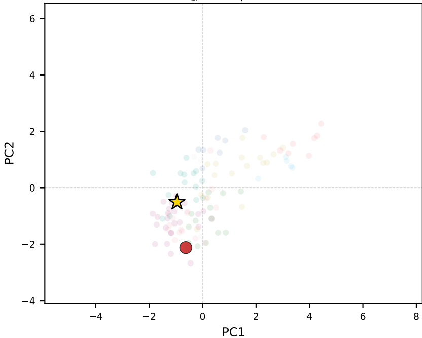
gpt-4o-mini | Zambia
