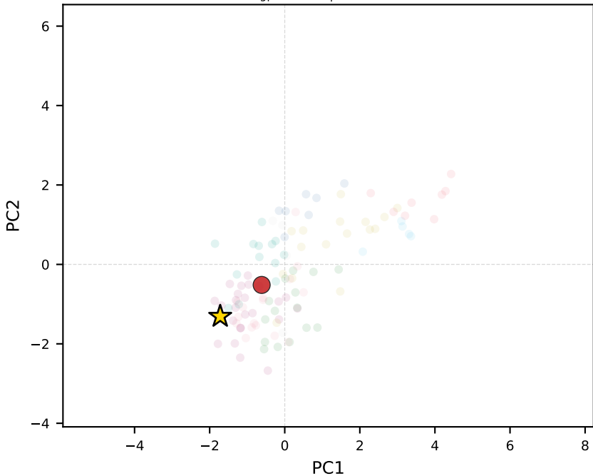
gpt-4o-mini | Zimbabwe
