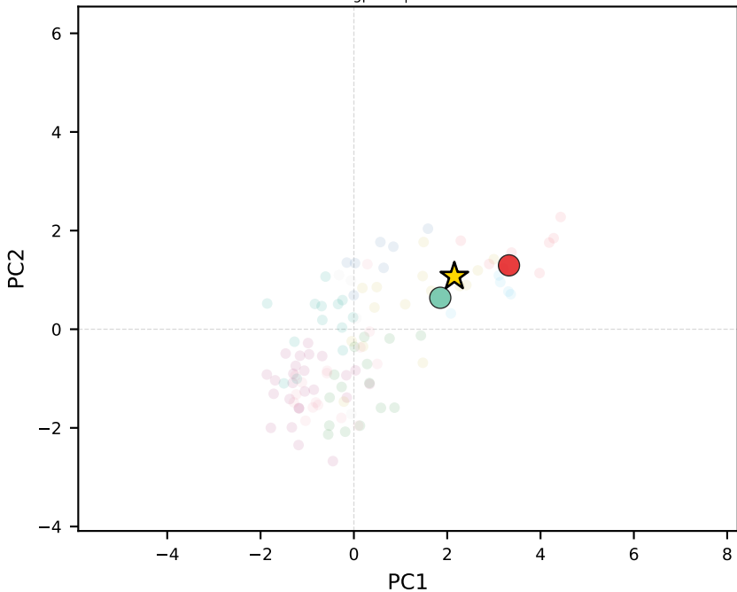
gpt-4o | Austria
