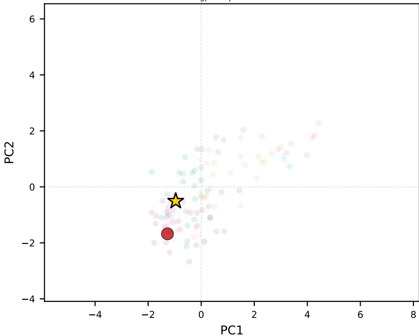
gpt-4o | Zambia
