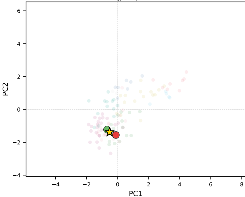
gpt-5.1 | Bolivia
