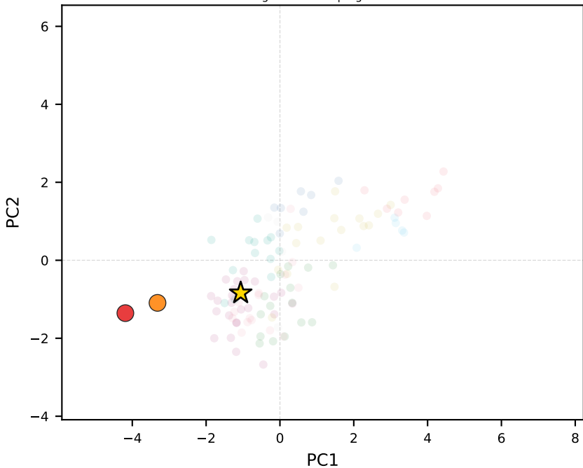
grok-4.1-fast | Algeria
