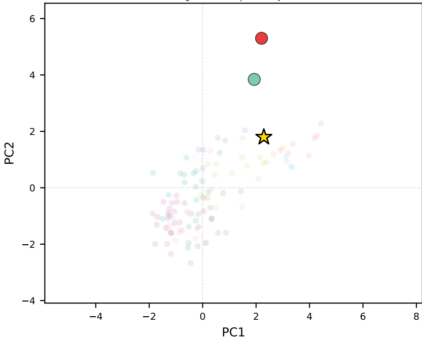
grok-4.1-fast | Germany
