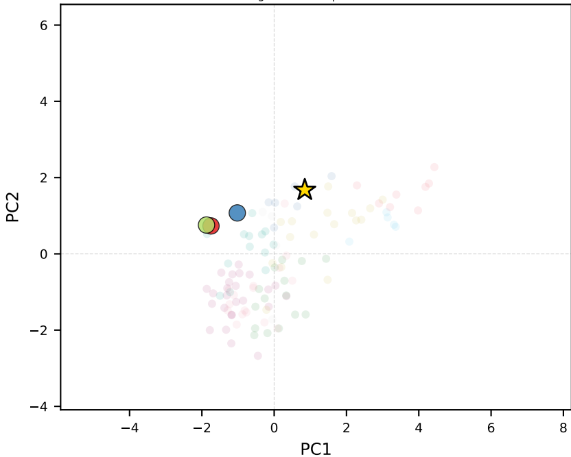
grok-4.1-fast | Macao
