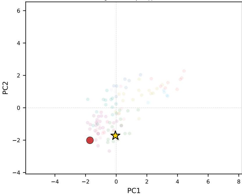
grok-4.1-fast | Philippines
