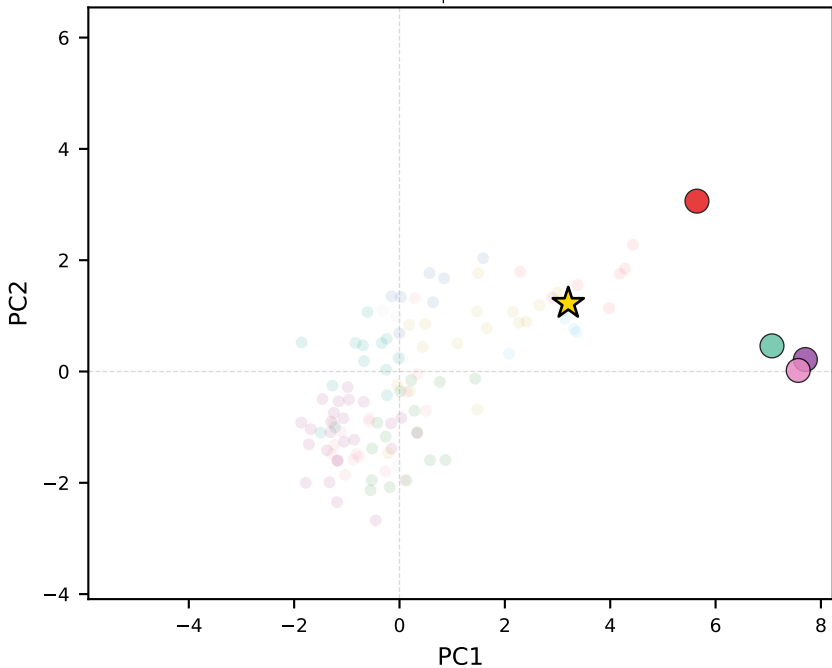
kimi-k2 | Switzerland
