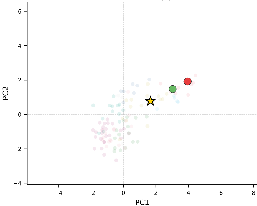
llama-3.3-70b-instruct | Spain
