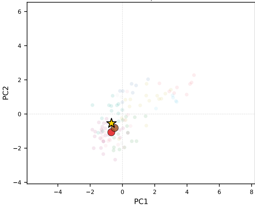
mistral-medium-3.1 | Kazakhstan
