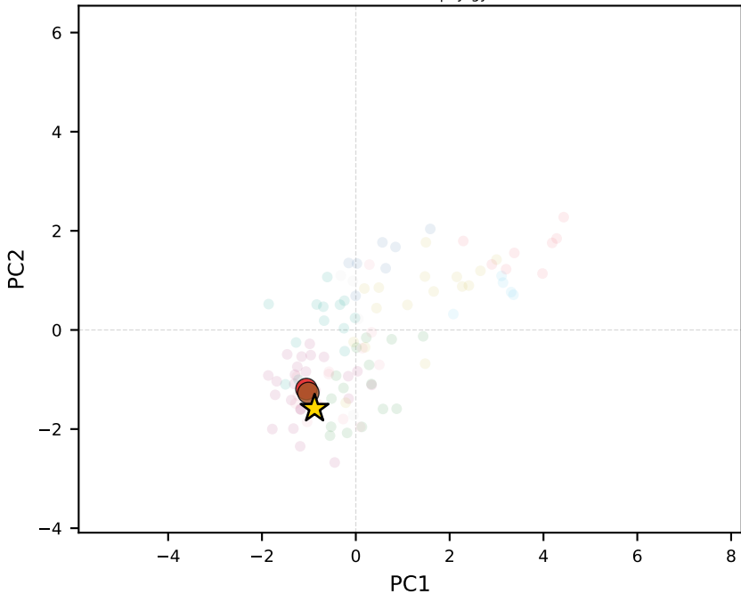
mistral-medium-3.1 | Kyrgyzstan
