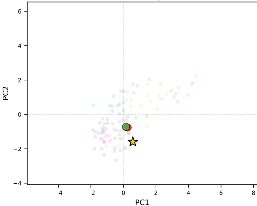
mistral-medium-3.1 | Mexico
