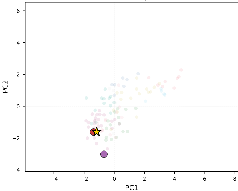
mistral-medium-3.1 | Rwanda
