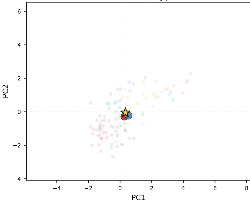
mistral-medium-3.1 | Singapore
