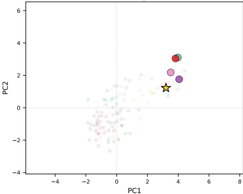
mistral-medium-3.1 | Switzerland
