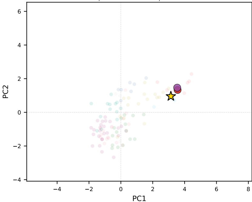
phi-3-mini-128k-instruct | Canada
