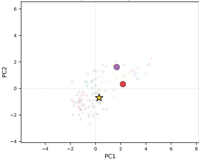
phi-3-mini-128k-instruct | Haiti
