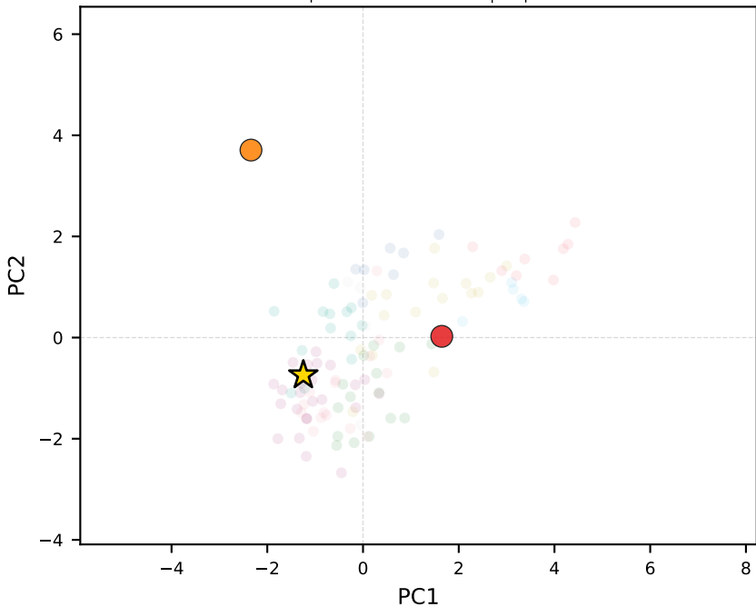
phi-3-mini-128k-instruct | Iraq
