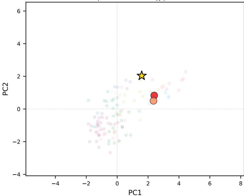
phi-3-mini-128k-instruct | Japan
