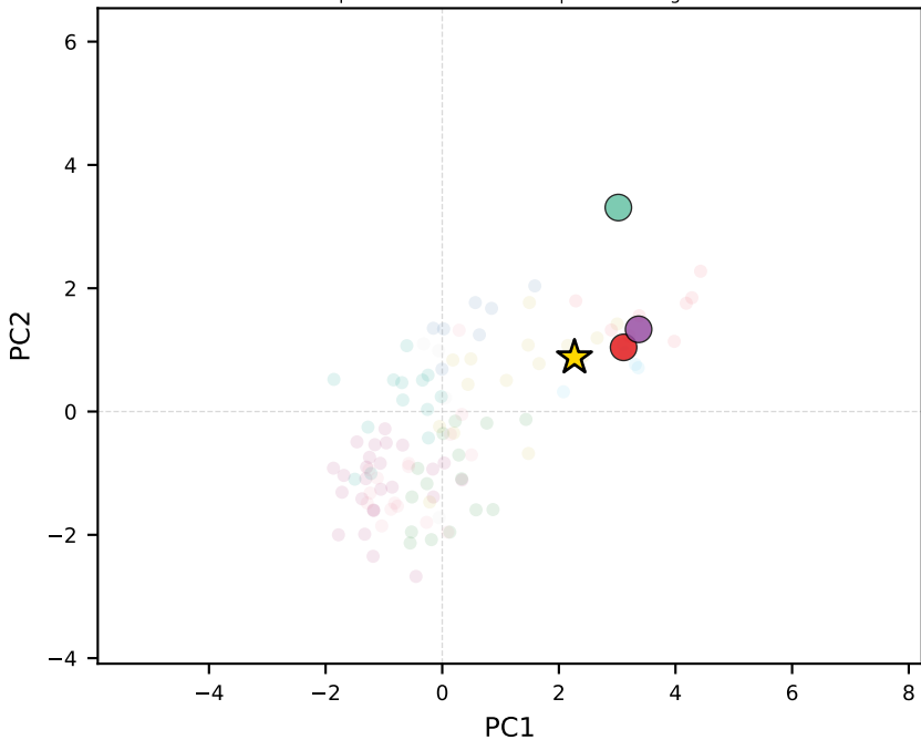
phi-3-mini-128k-instruct | Luxembourg
