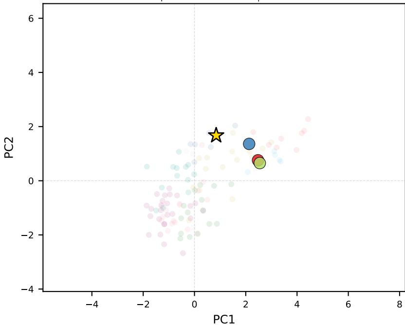
phi-3-mini-128k-instruct | Macao
