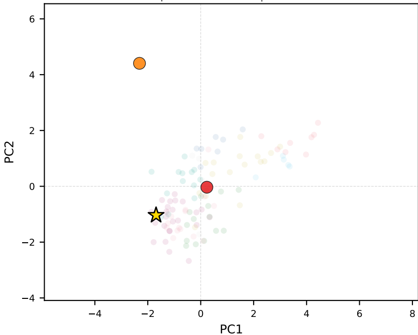
phi-3-mini-128k-instruct | Palestine
