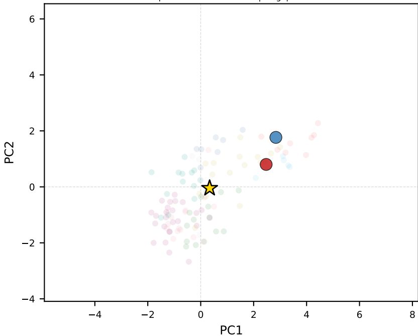
phi-3-mini-128k-instruct | Singapore
