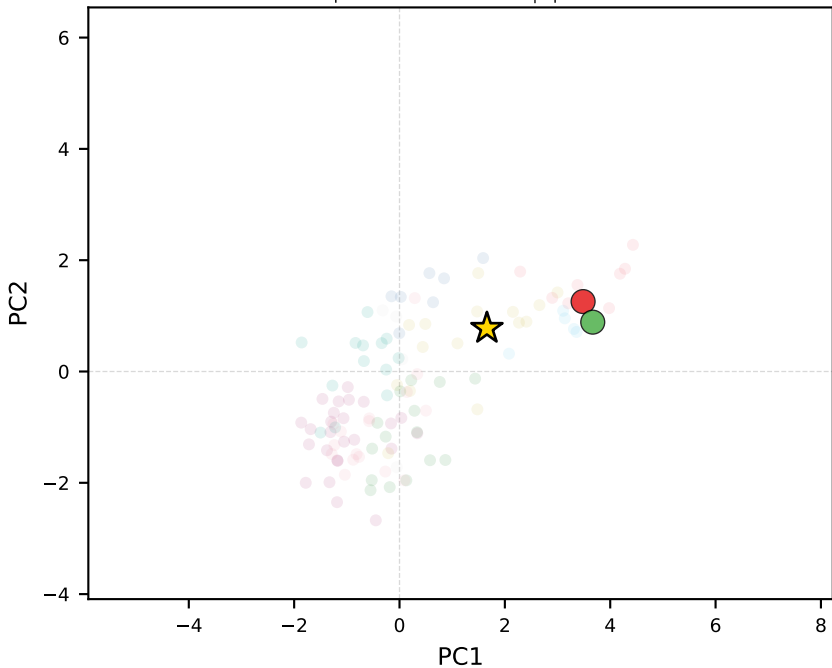
phi-3-mini-128k-instruct | Spain
