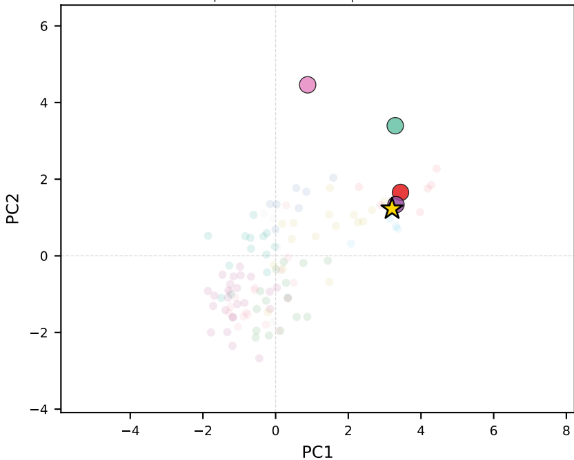
phi-3-mini-128k-instruct | Switzerland
